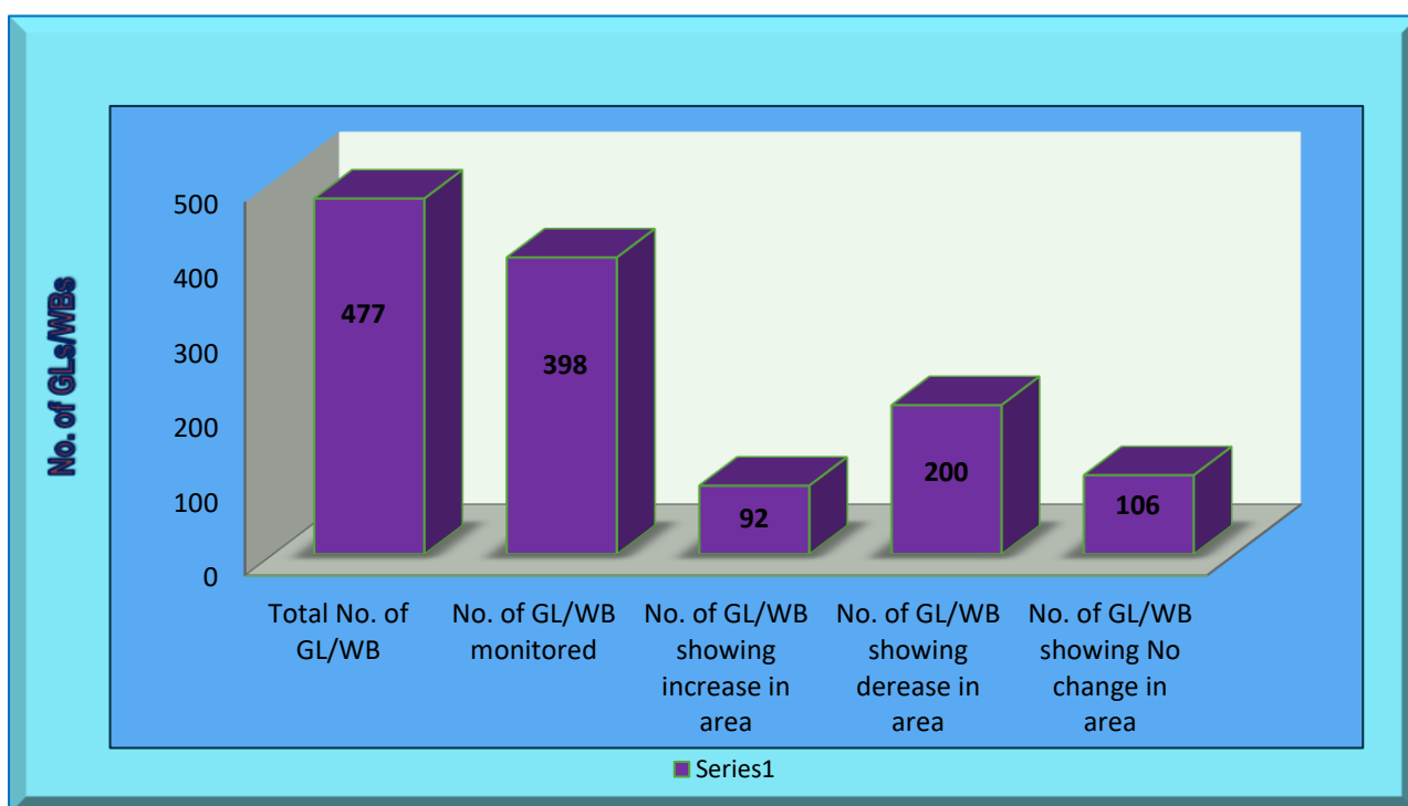
Figure 2: Glacial Lakes/ Water Bodies Monitored during the month September 2021
