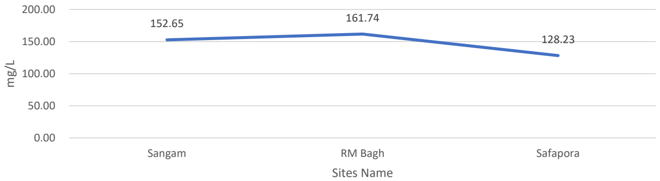
Total Hardness variation along the Jhelum River
