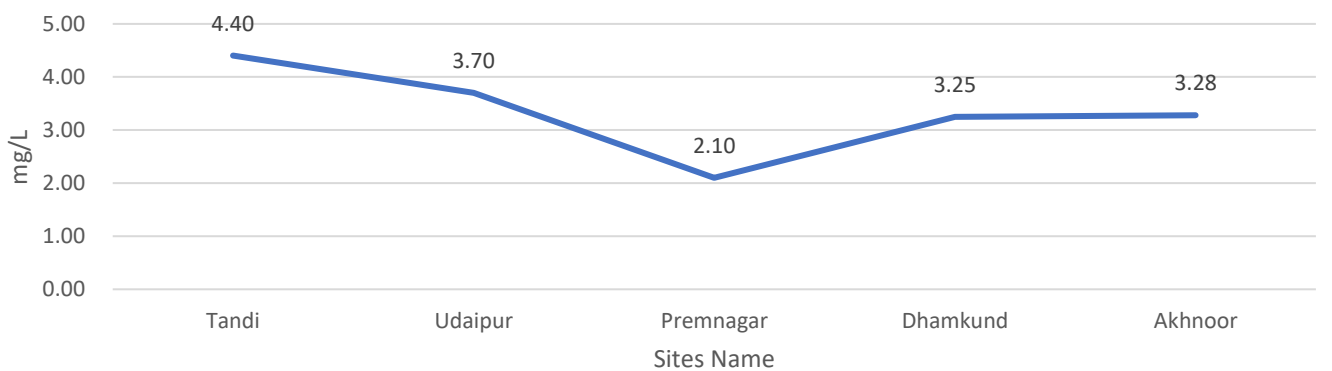
NO 3 -N Variation along the Chenab River
