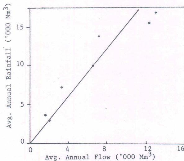
FIG. 12 PLOT OF ANNUAL RAINFALL Vs. ANNUAL FLOW
